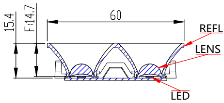
OPTICAL ASSEMBLY DIAGRAM
